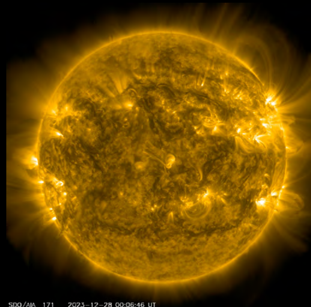
SDO/AIA 171 2023-12-28 00:06:46 UT
